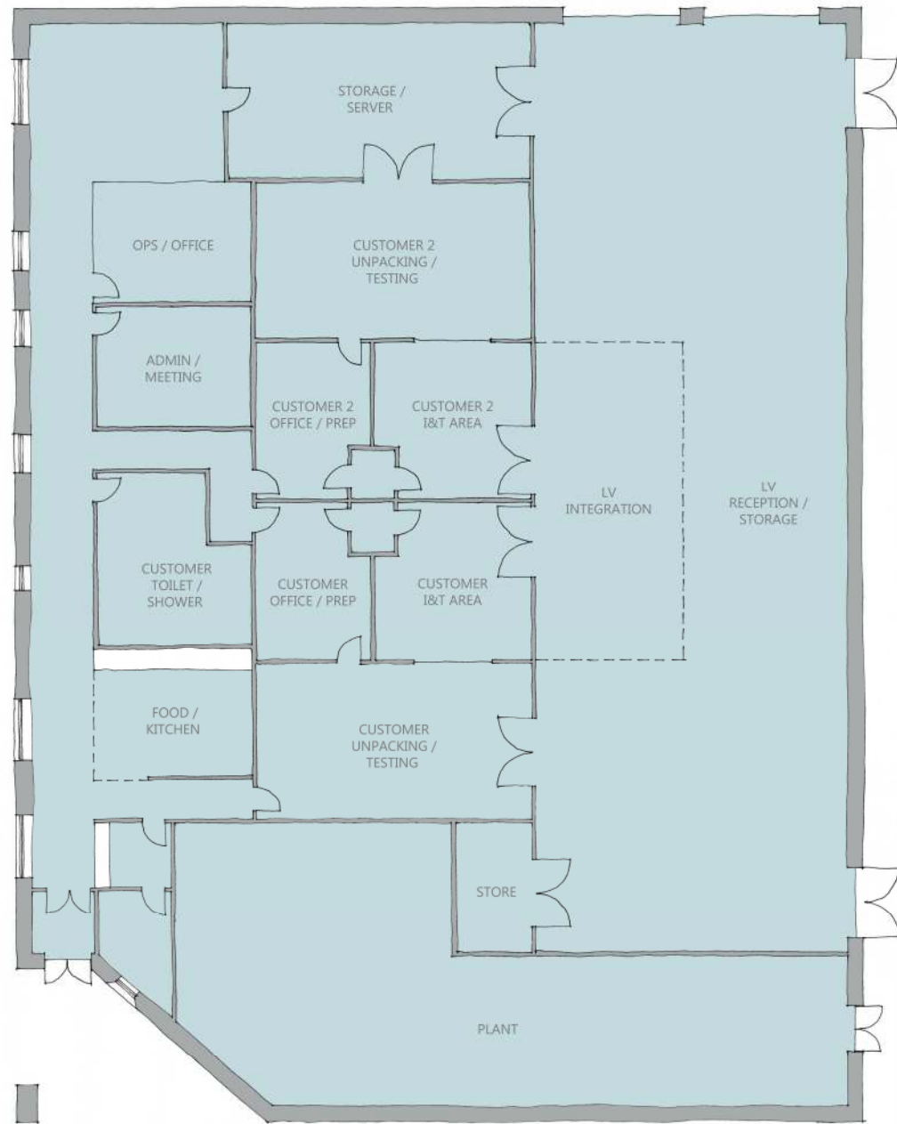
FLOOR PLAN AS PROPOSED
